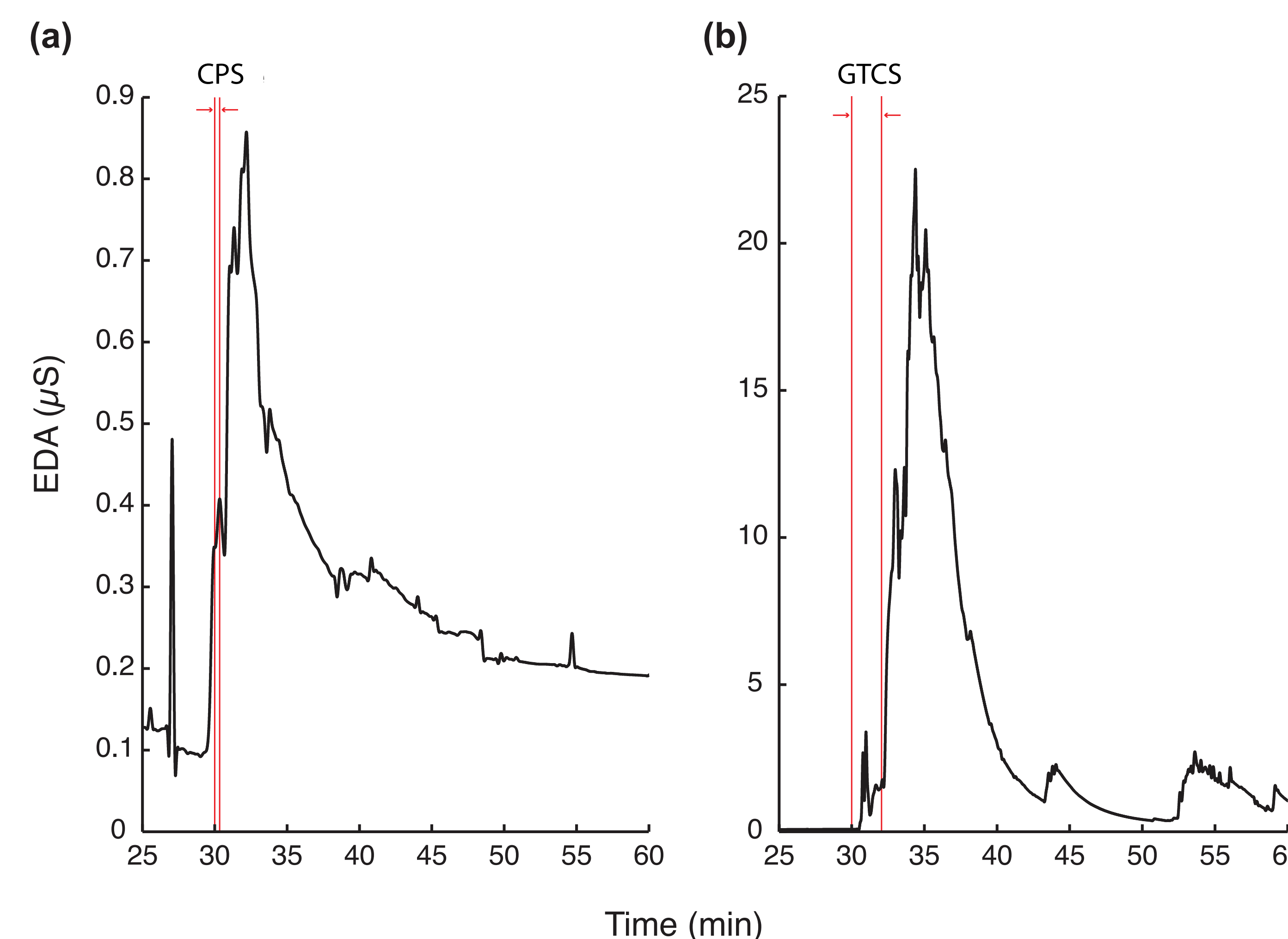
Figure 3. Example of EDA changes during (a) a complex partial seizure (CPS) (b) secondarily generalized tonic-clonic seizure (GTCS)
