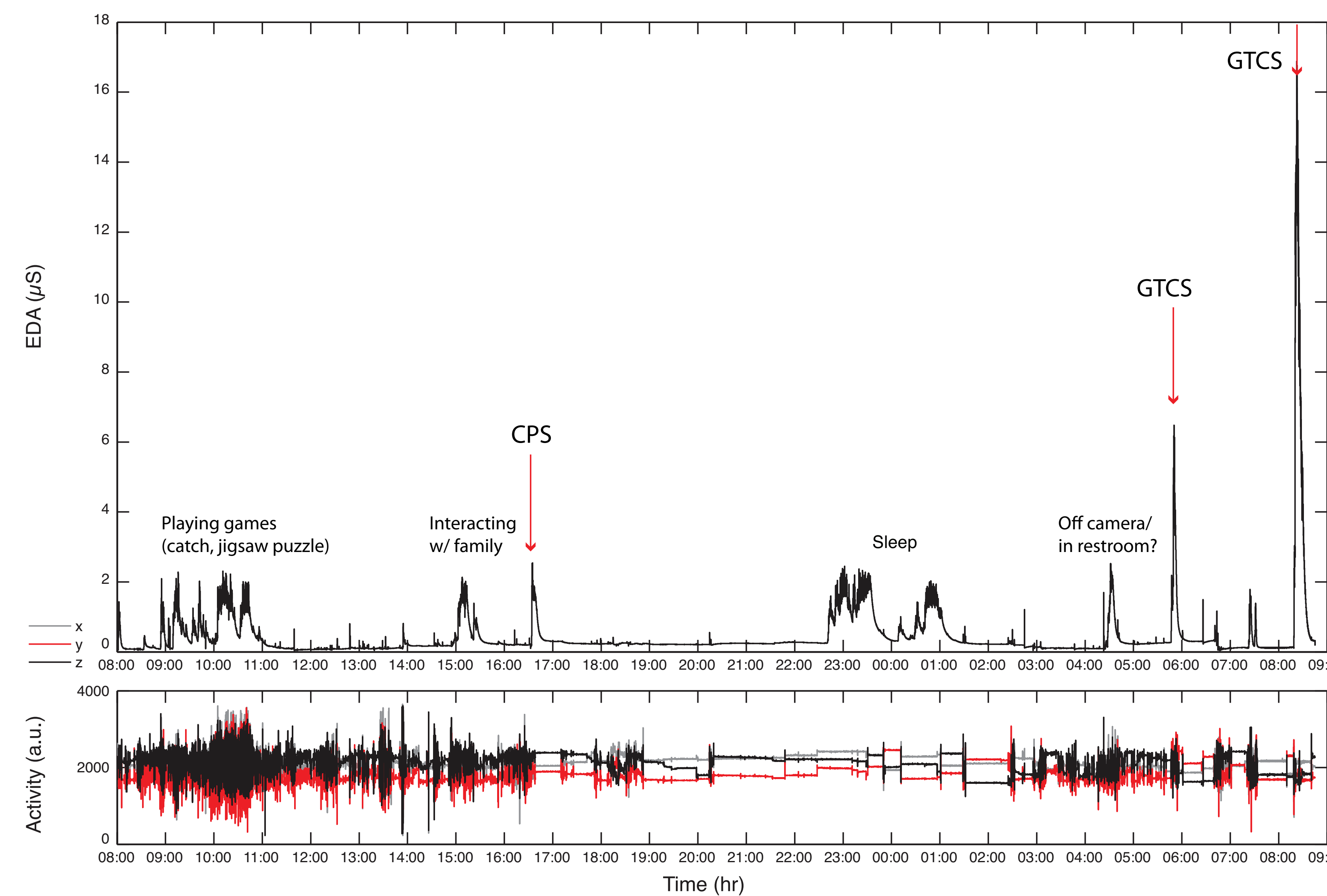
Figure 2. Example of a 24-hour EDA recording from an 11 y.o. girl with intractable epilepsy.
