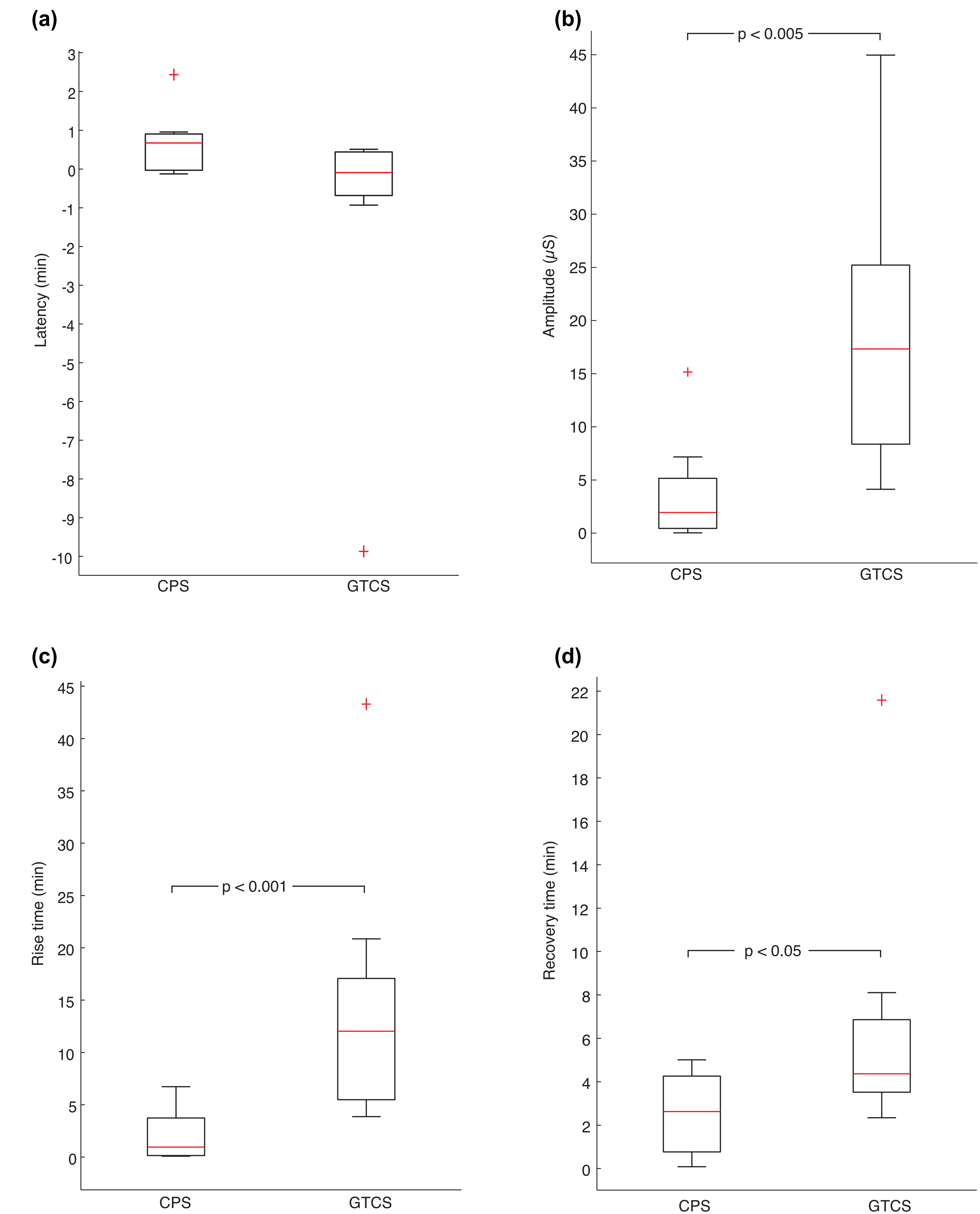
Figure 4. Periictal EDA parameters. (a) Latency (b) Amplitude (c) Rise time (d) Recovery time
